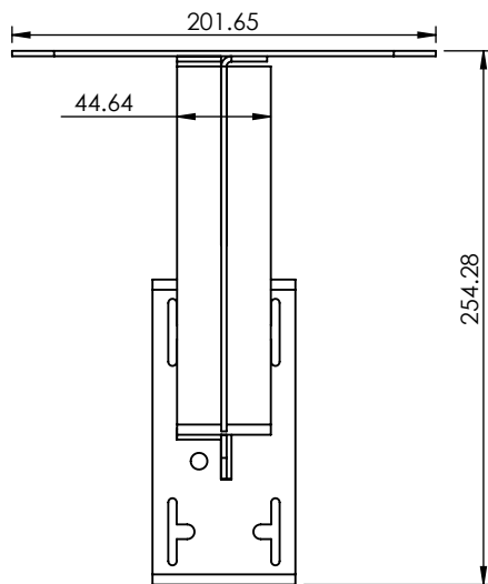
Vista frontal
